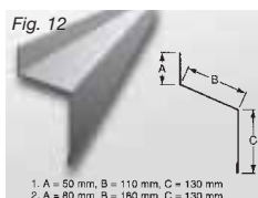
Fig. 12 Droppbleck över skjutport 1. A = 50 mm, B = 110 mm, C = 130 mm 2. A = 80 mm, B = 180 mm, C = 130 mm
